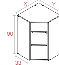
Corner Module with Chamfered Corner H90
